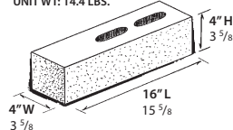
4" REGULAR - CORE PATTERN 2 UNIT WT: 14.4 LBS.
