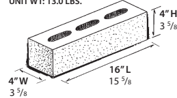
4" REGULAR - CORE PATTERN 3 UNIT WT: 13.0 LBS.
