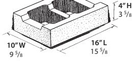
10" RESTRICTED BOTTOM BOND BEAM UNIT WT: 19.4 LBS.
