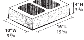
10" PILASTER UNIT WT: 22.1 LBS.
