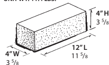
4" UTILITY SIZE - SOLID UNIT WT: 11.4 LBS.
