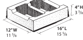
12" RESTRICTED BOTTOM BOND BEAM UNIT WT: 22.1 LBS.
