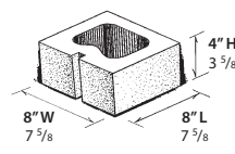
8" HALF UNIT / SASH UNIT WT: 10.4 LBS.
