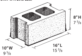
6" STRETCHER UNIT WT: 29.0 LBS.
