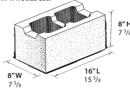
8" RESTRICTED BOTTOM BOND BEAM UNIT WT: 36.25 LBS.
