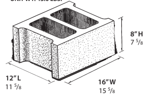
12" STRETCHER UNIT WT: 43.0 LBS.
