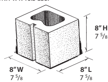
8" HALF UNIT/SASH UNIT WT: 18.5 LBS.
