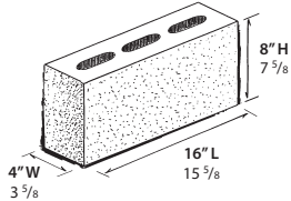
4" REGULAR UNIT WT: 24.0 LBS.
