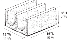
12" SOLID BOND BEAM UNIT WT: 60.5 LBS.
