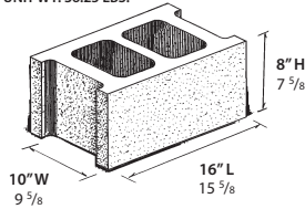
8" STRETCHER UNIT WT: 36.25 LBS.
