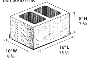
10" PILASTER UNIT WT: 43.0 LBS.
