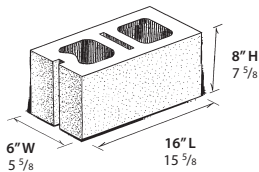
6" CORNER / SASH UNIT WT: 29.0 LBS.
