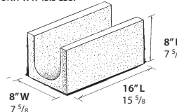
8" SOLID BOND BEAM UNIT WT: 43.5 LBS.
