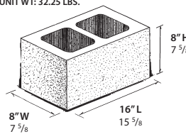
8" PILASTER UNIT WT: 32.25 LBS.
