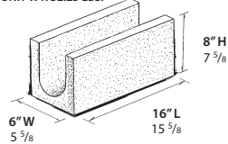
6" SOLID BOND BEAM UNIT WT: 32.25 LBS.
