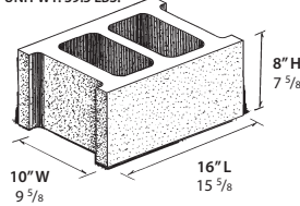
10" STRETCHER UNIT WT: 39.5 LBS.
