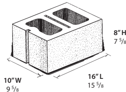
10" CORNER / SASH UNIT WT: 39.5 LBS.
