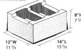
12" RESTRICTED BOTTOM BOND BEAM UNIT WT: 50.0 LBS.
