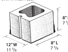
12" HALF UNIT/SASH UNIT WT: 25.4 LBS.
