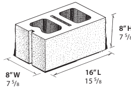
8" CORNER / SASH UNIT WT: 36.25 LBS.
