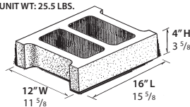
12" STRETCHER UNIT WT: 25.5 LBS.
