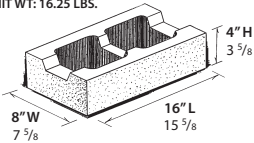
8" RESTRICTED BOTTOM BOND BEAM UNIT WT: 16.25 LBS.
