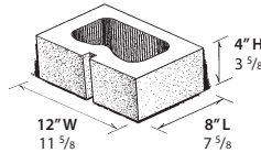
12" HALF UNIT/SASH UNIT WT: 13.0 LBS.
