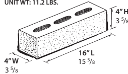
4" REGULAR - CORE PATTERN 3 UNIT WT: 11.2 LBS.
