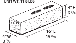
4" REGULAR - CORE PATTERN 2 UNIT WT: 11.8 LBS.
