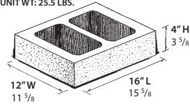
12" PILASTER UNIT WT: 25.5 LBS.
