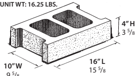
8" STRETCHER UNIT WT: 16.25 LBS.
