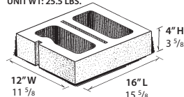
12" CORNER / SASH UNIT WT: 25.5 LBS.
