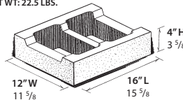
12" RESTRICTED BOTTOM BOND BEAM UNIT WT: 22.5 LBS.
