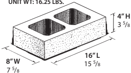
8" PILASTER UNIT WT: 16.25 LBS.
