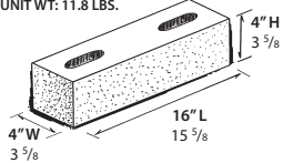
4" REGULAR - CORE PATTERN 1 UNIT WT: 11.8 LBS.
