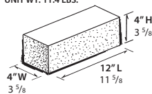
4" UTILITY SIZE - SOLID UNIT WT: 11.4 LBS.
