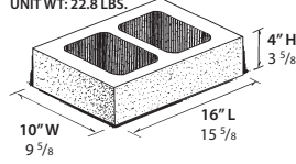
10" PILASTER UNIT WT: 22.8 LBS.
