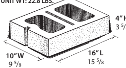
10" CORNER / SASH UNIT WT: 22.8 LBS.
