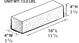
4" REGULAR - SOLID UNIT WT: 13.0 LBS.
